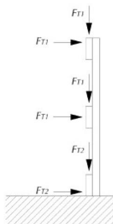
Figure 6 — Charges de service, alternative 1 Charges agissant séparément
